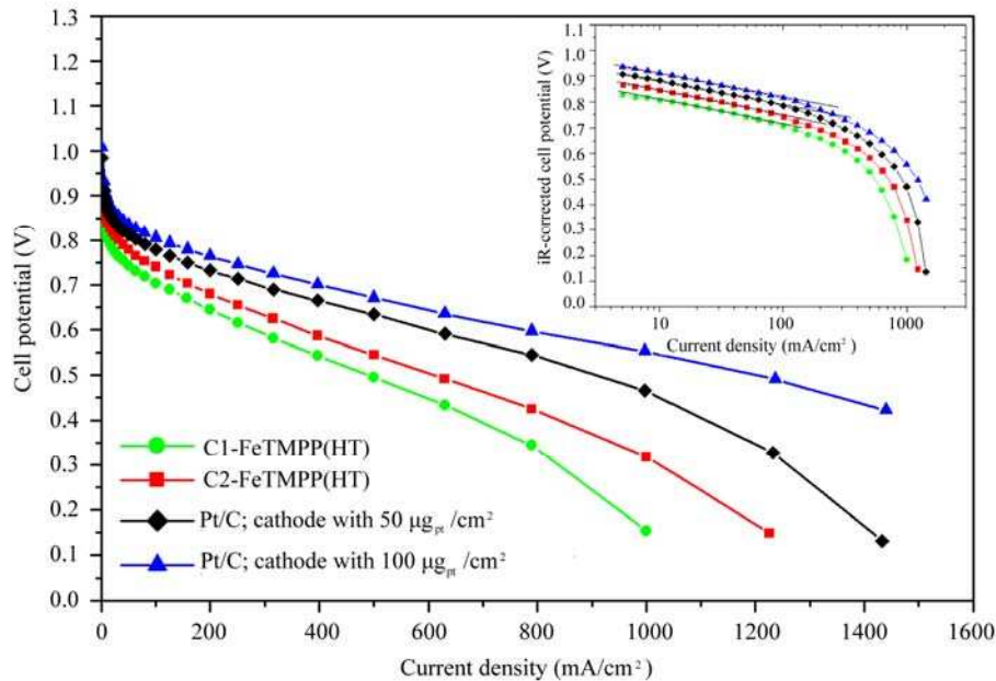
Figure 7. Single-cell PEMFC performance of C1-FeTMPP(HT), C2-FeTMPP(HT), and Pt/C oxygen reduction electrodes at 353 \text{ K} Anode: 0.4 \text{ mg}_{\text{Pt}}/\text{cm}^2 and cathode: 50 \mu\text{g}_{\text{Fe}}/\text{cm}^2 . For comparison, performance of Pt/C as cathode with 50 or 100 \mu\text{g}_{\text{Pt}}/\text{cm}^2 also shown. Inset shows the Tafel plots for the catalysts.
