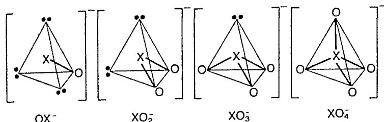
Figure 16.9 Structures of the oxoacids.
