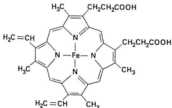
Figure 15.15 Structure of haem.
