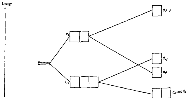
Figure 7 19 Tetragonal distortion
