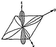
Figure 7 18 d^8 arrangement strong field (The d_{z^2} orbital is full, the d_{x^2-y^2} empty)
