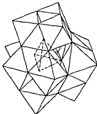
Figure 22.10 12 polyacid e.g. \text{H}_4[\text{PO}_4 \cdot \text{W}_{12}\text{O}_{36}] (From H.J. Emeleus and A.G. Sharpe, Modern Aspects of Inorganic Chemistry 4th ed. RKP 1973)
