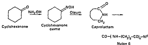
Figure 14 5 Nylon-6
