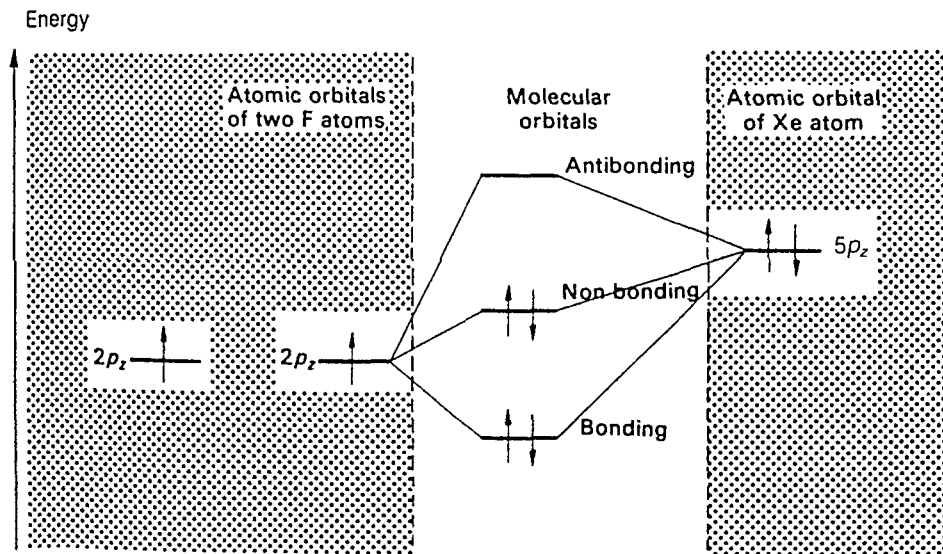
Figure 17.4 Molecular orbitals in XeF 2 .
