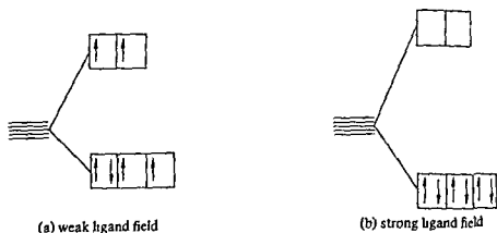
Figure 24.4 Electronic arrangements of the d^6 ion Fe^{2+}
