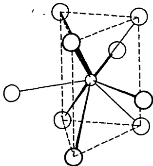
Figure 23.6 Structure of the enneaheptahydridorhenium(VII) ion [\text{ReH}_9]^{2-}
