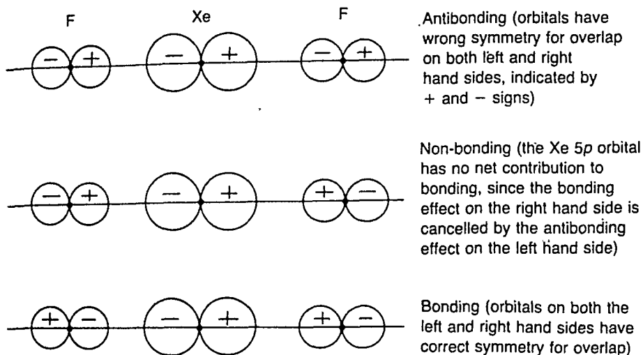
Figure 17.3 Possible combinations of atomic orbitals in XeF 2 .
