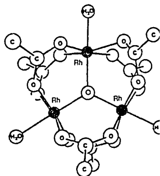
Figure 25.8 Structure of [Rh_3O(CH_3COO)_6(H_2O)_3]^+
