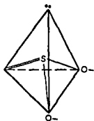
Fig 15.9 Structure of sulphite ion \text{SO}_3^{2-}
