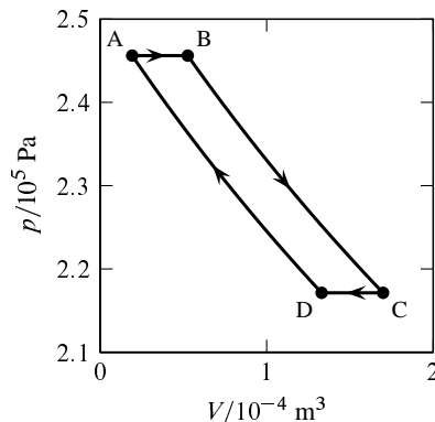
Figure 4.4 Indicator diagram for a Carnot engine using \text{H}_2\text{O} as the working substance. In this example, T_h = 400 \text{ K} , T_c = 396 \text{ K} , \epsilon = 1/100 , w = -1.0 \text{ J} . In state A, the system consists of one mole of \text{H}_2\text{O}(l) . The processes (all carried out reversibly) are: A \rightarrow B, vaporization of 2.54 mmol \text{H}_2\text{O} at 400 K; B \rightarrow C, adiabatic expansion, causing vaporization of an additional 7.68 mmol; C \rightarrow D, condensation of 2.50 mmol at 396 K; D \rightarrow A, adiabatic compression returning the system to the initial state.
