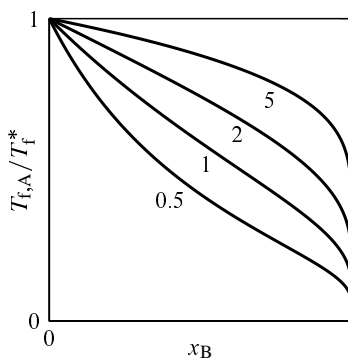
Figure 12.5 Freezing-point curves of ideal binary liquid mixtures. The solid is component A. Each curve is calculated from Eq. 12.5.4 and is labeled with the value of \Delta_{\text{fus,A}}H/RT_{f,A}^* .
