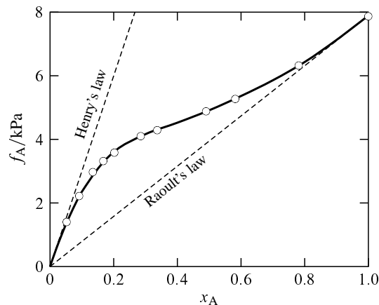
Figure 9.8 Fugacity of ethanol in a gas phase equilibrated with a binary liquid mixture of ethanol (A) and H 2 O at 25 °C and 1 bar. Open circles: experimental measurements. a The dashed lines show Henry's law behavior and Raoult's law behavior.
