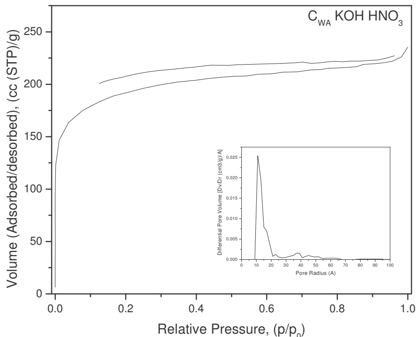
Fig. 23. N 2 adsorption-desorption isotherms of carbon materials prepared from Limonea Acidissima ; the corresponding pore size distribution of the activated carbon material is shown in the insert (reproduced from ref. 178]
